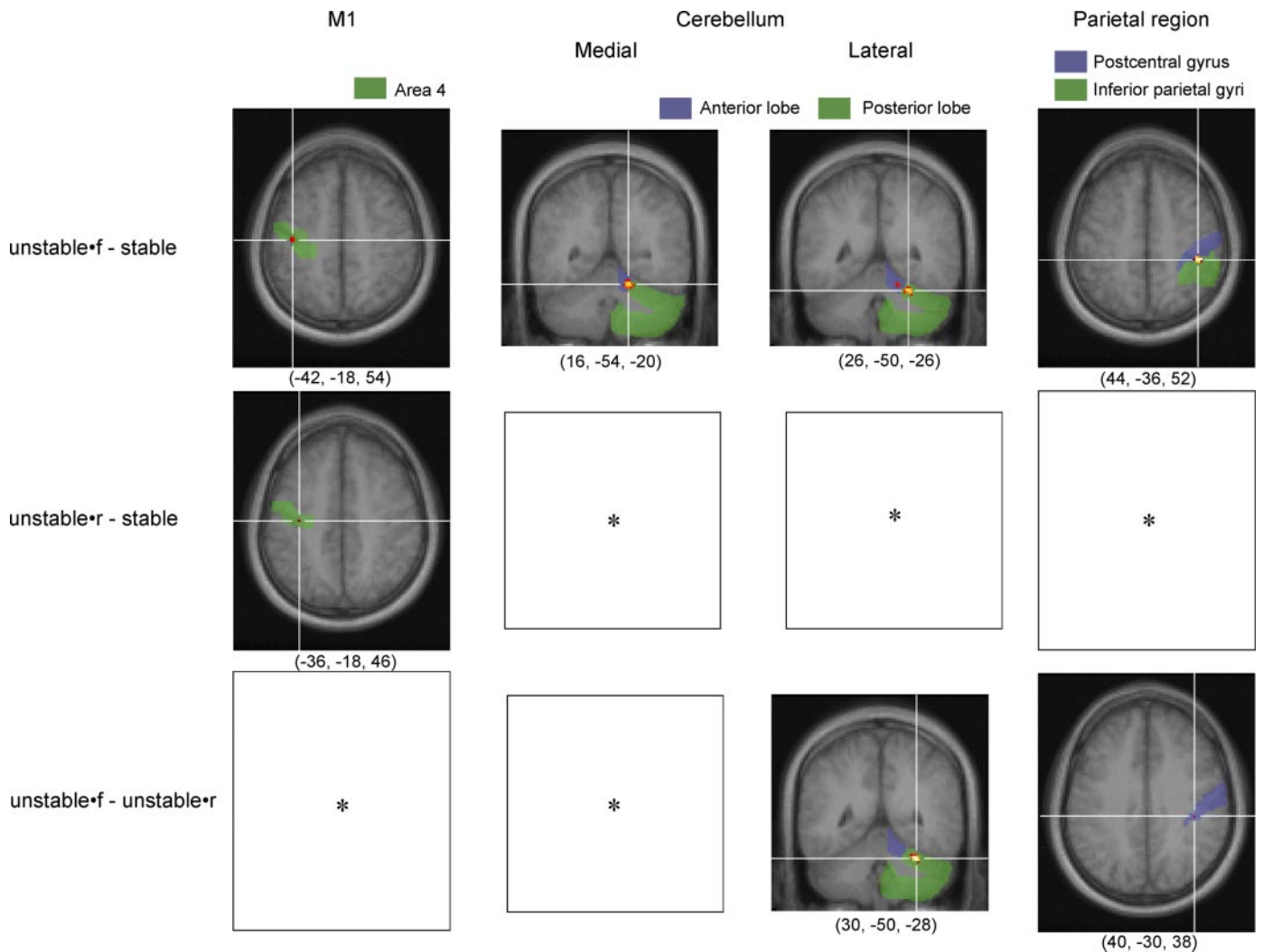
FIG. 3. ROI masks (blue and green regions) and foci of activity for the unstable·f-stable contrast ( top ), the unstable·r-stable contrast ( middle ), and the unstable·f-unstable·r contrast ( bottom ). Asterisks (*) indicate that there was no significant activation in the corresponding region. Anatomical images were normalized and averaged across subjects. Transverse slices corresponding to locations of local maxima are shown for M1 and inferior parietal lobule; coronal slices are shown for cerebellum. Coordinates of local maxima shown below each slice correspond to those listed in Table 3.
